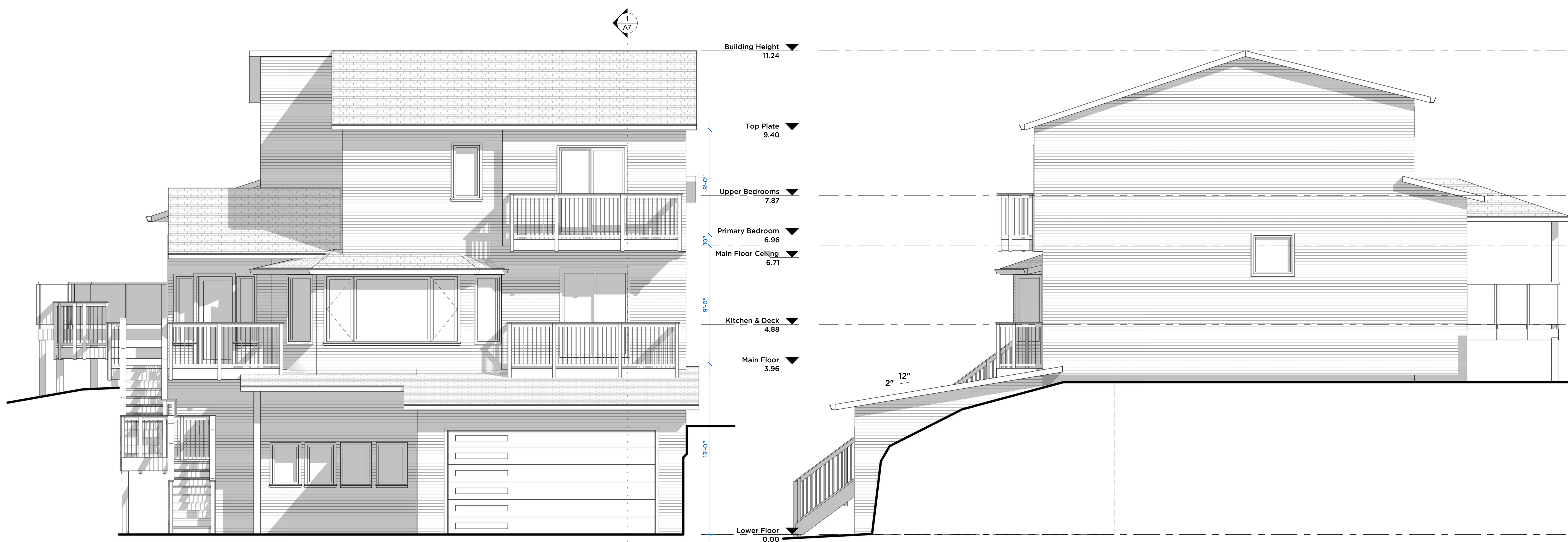
② RIGHT (North) 1/4" = 1'-0"
